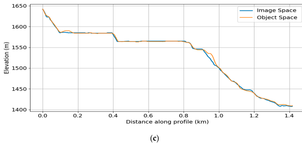
Figure 9. (a) Shaded DEM of the Morenci Mine are computed using SGM in the image space from tri-stereo SkySat images acquired on 1 January 2019; (b) Example of sub-scenes covering the area. (c) Profile along the transect (AA') extracted from image space DEM and object space DEM.
