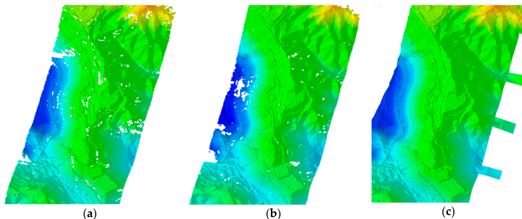
Figure 8. Subset of SkySat shaded DEMs over Morenci Mine using (a) backward and nadir images, (b) nadir and forward images, (c) backward, nadir and forward images.
