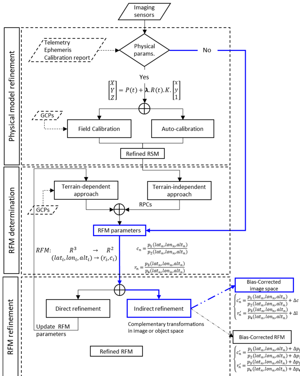
Figure 1. Workflow for image geometry refinement including physical model (Rigorous Sensor Model) and rational function model (RFM) approaches. The blue color pathway shows the processing path described in this study and is added as an additional module in the COSI-Corr package.
