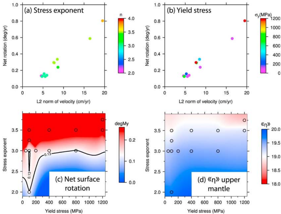
Figure 8. (a) Resulting net rotation and volume L_2 norm of velocity, color coded by stress exponent. (b) Same quantity, color coded by yield stress. (c) Net surface rotation as function of stress exponent and yield stress. (d) Integrated viscosity « \eta » in the upper mantle as function of stress exponent and yield stress.
