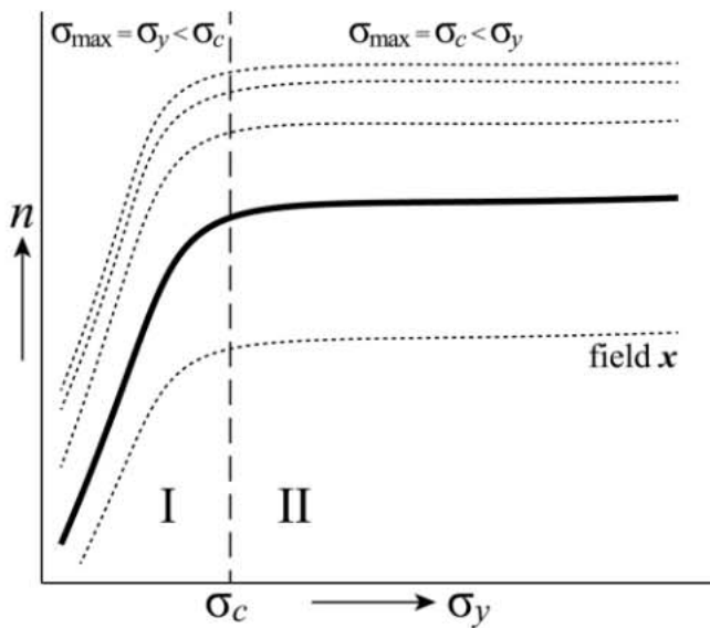
Figure 5. Schematic of the behavior of a resulting quantity as function of (s_y, n) . Contour lines of the field x are indicated; the two domains are denoted with I and II. The convective stress is s_c .
