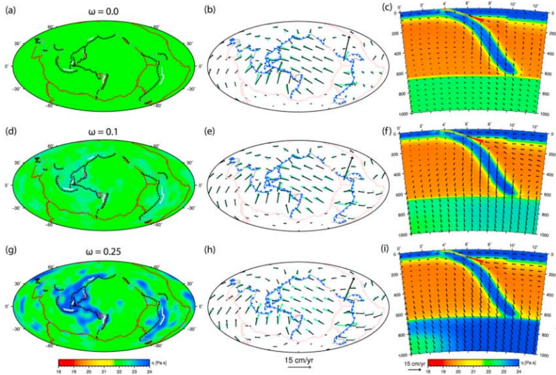
Figure 9. (a–c) Case 13, lower mantle tomography conversion factor w = 0.0 ; (d–f) Case 2 with factor w = 0.1 ; (g–i) Case 14, factor w = 0.25 . (left) Viscosity field at 700 km depth (color map), with slab contours at 600 km depth plotted in white contours. The contours are defined by nondimensional temperature T = 0.55 . (middle) Global plate motions, NNR_NUVEL1A plate motions are plotted in green, Rhea velocities in black. (right) Cross-sections through Peru (for location see P2, Figure 1). The background is viscosity; the vectors show velocity.
