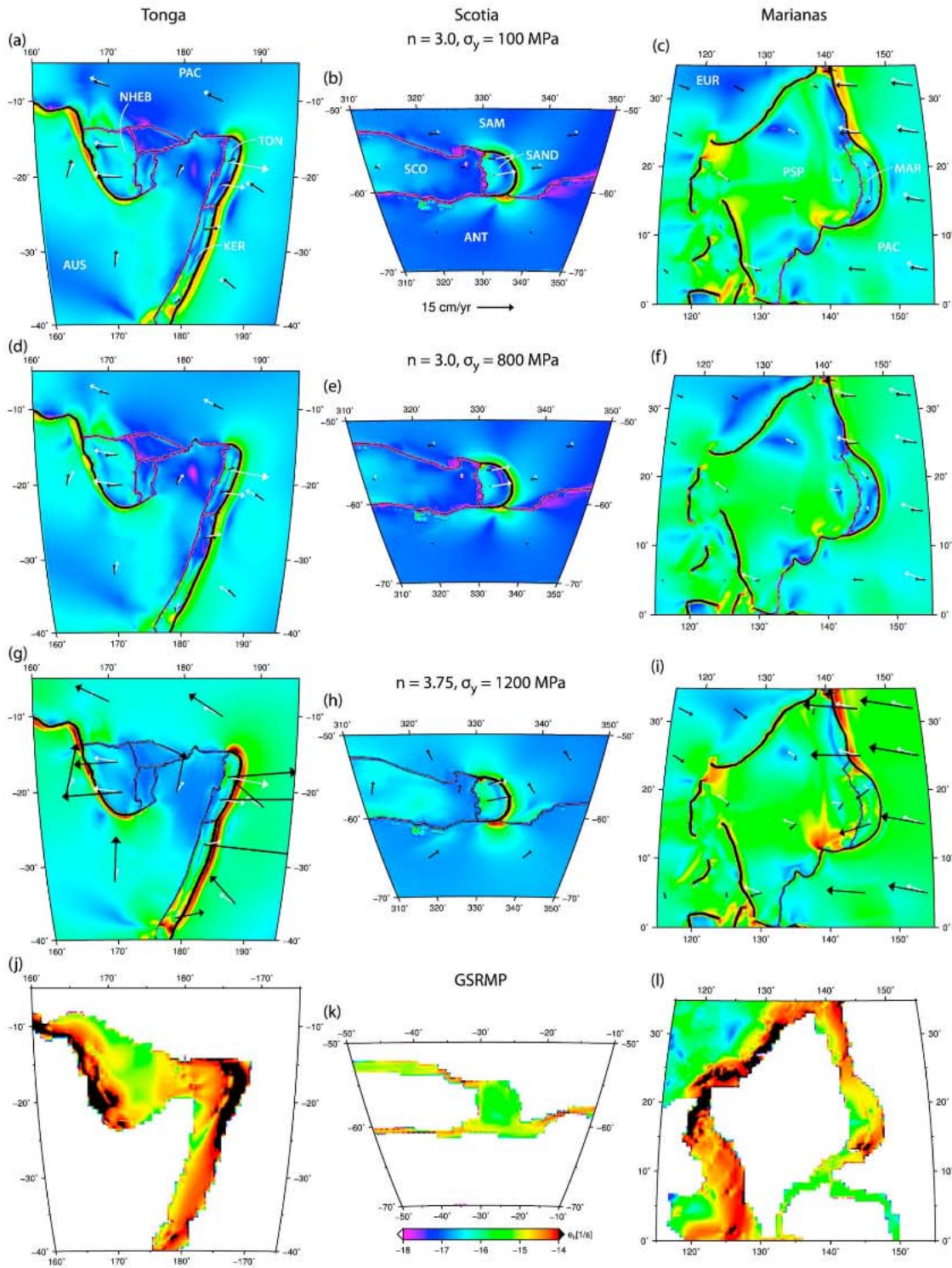
Figure 10. Comparison of surface strain rates. (left to right) Tonga, Scotia, Marianas. (top to bottom) Case 2, s_y = 100 MPa and n = 3.0 ; Case 5, s_y = 800 MPa, n = 3.0 ; Case 12, s_y = 1200 MPa, n = 3.75 ; Global Strain Rate Map Project [Kreemer et al., 2003]. NNR_NUVELIA plate motions are shown in white, Rhea velocities in black; plotted on top of the second invariant of the strain rate tensor.
