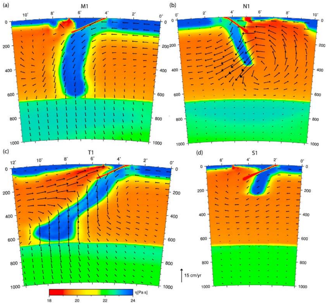
Figure 15. Cross-sections through slabs and microplates of Case 2, with stress exponent n = 3.0 and yield stress s_y = 100 MPa. Arrows: velocity; background color: viscosity. (a) Marianas, M1; (b) New Hebrides, N1; (c) Tonga, T1; (d) Sandwich, S1.
