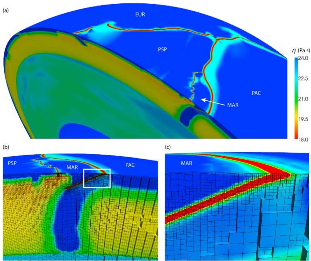
Figure 2. (a) Cutout showing viscosity in a global model with stress exponent n = 3.0 and yield stress s_y = 100 MPa (Case 2) through the Marianas and Philippines. (b) Zoom-in on viscosity of the Marianas subduction zone, showing the mesh. (c) Further zoom-in on the hinge of the Marianas slab, as denoted by the white box in Figure 2b. Plate labels are: EUR: Eurasia; MAR: Marianas; PAC: Pacific; PSP: Philippine Sea.
