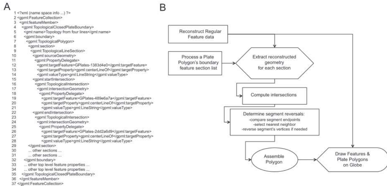
Fig. 3. Details associated with the CCP algorithm as implemented within GPlates. (A) Sample GPML file that illustrates how several Line features (lines 12, 19, and 26) are contained within a TopologicalClosedPlateBoundary. (B) Processing sequence associated with reconstructing and resolving a previously created TopologicalClosedPlateBoundary.
