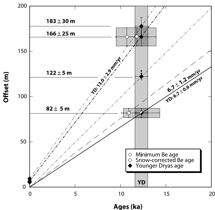
Figure 11. Slip rate diagram using the different ages estimates of the uncorrected and snow-corrected surface exposure ages (Table 2), and of the Younger Dryas (YD) [Alley et al. , 1993; Alley, 2000]. Arrows for 122 \pm 5 m indicate that this offset is a minimum bound. Dash lines represent the various slip rates derived from each dated offsets (see Table 2). Bold dash lines with slip rate values are best estimated (see text for detail).
