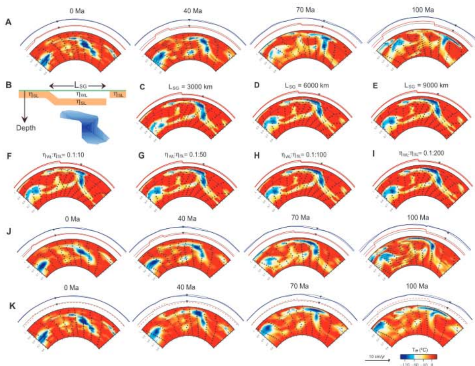
Figure 4. Subduction modeling with inverse method. All cross sections are at 41^{\circ}\text{N} , with the velocity vectors (black arrows) plotted over the temperature field (in color). Dynamic topography (blue) and plate motions (red) along the profile are shown above the cross section. The black triangle denotes a borehole site ( 41.6^{\circ}\text{N} , 254^{\circ}\text{E} ) that moves with the continent. All runs have a lower mantle viscosity h_{LM} = 15 , h_{UM} = 1 and an effective temperature anomaly T_e = 160^{\circ}\text{C} . (a) An SBI run with a standard mantle model from present-day mantle structure leads to unrealistic subduction geometry back in time, indicating the requirement of a stress guide. (b) A sketch of the parameterized stress guide showing an imposed small viscosity ( h_{WL} ) layer overlying a large viscosity ( h_{SL} ) layer underneath the continent, where L_{SG} indicates the length of the guide. The recovered slab at 70 Ma (c–e) with the different values of L_{SG} and (f–i) with various viscosity ratios (relative to 10^{21} Pa s) within the two layers, showing the solutions converge as long as L_{SG} > 3,000 km and h_{WL} : h_{SL} < 0.1:50 . (j) The evolution of the slab after five forward adjoint iterations including a stress guide with L_{SG} = 6,000 km and h_{WL} : h_{SL} = 0.1:100 , where reasonable subduction geometry develops. (k) A free convection test showing that without the imposed plate motions and stress guide, the slab has almost the same vertical velocities as can be seen from the depth of the structure at different times.
