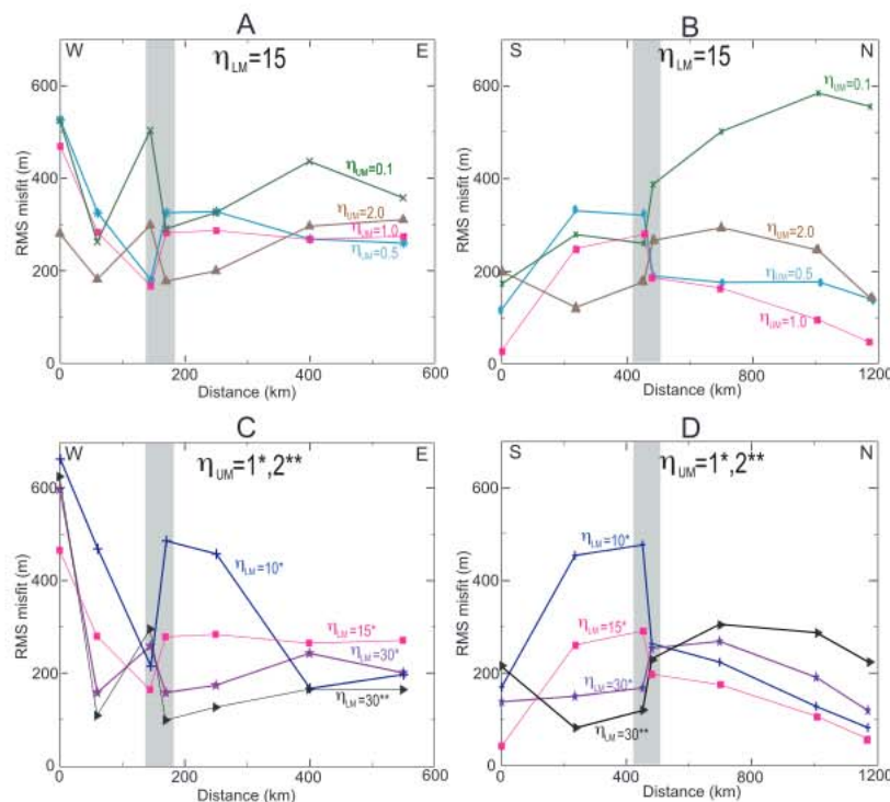
Figure 6. RMS amplitude misfit between observed and model borehole tectonic subsidence. (a and b) Misfit for models with constant lower mantle viscosity h_{LM} = 1.5 \times 10^{22} Pa s. (c and d) Misfit for models with upper mantle viscosity h_{LM} = 1-2 \times 10^{21} Pa s. Grey vertical bar indicates intersection of N-S and E-W profiles. All viscosity values are shown with respect to reference viscosity of 10^{21} Pa s.
