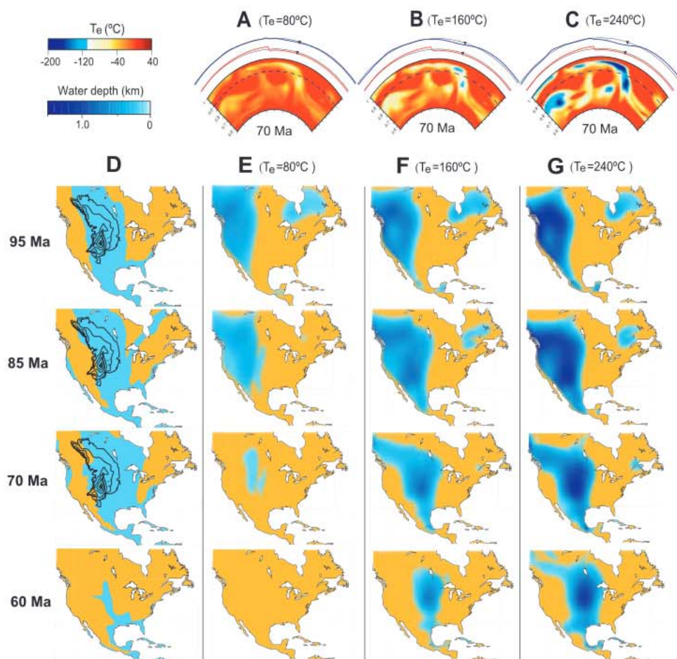
Figure 5. Selection of the effective temperature through flooding predictions. (a–c) Recovered Farallon slab at 70 Ma with three different magnitudes of temperature anomaly (80, 160, and 240^\circ\text{C} , respectively) and lower mantle viscosities largely traded off with temperature ( 7 \times 10^{21} , 15 \times 10^{21} , and 30 \times 10^{21} Pa s, respectively; all cases have an upper mantle viscosity of 10^{21} Pa s), where all three models see the same slab geometries. (d) Reconstructed WIS flooding (blue [Smith et al. , 1994]) and sediment isopachs (black contours with 2,000 ft contour interval [Cook and Bally, 1975]). (e–g) The predicted Late Cretaceous flooding with different T_e , with the 160^\circ\text{C} temperature anomaly (Figure 5f) matching observations (Figure 5d) to the best extent.
