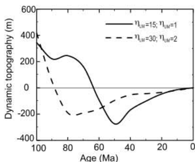
Figure 13. Time-dependent predictions of dynamic subsidence for East Lake Athabasca region (coordinates 108°W, 59°5′N) for two dynamic models. Values of upper mantle viscosity \eta_{UM} and lower mantle viscosity \eta_{LM} are given with respect to reference value of 10^{21} Pa s.
