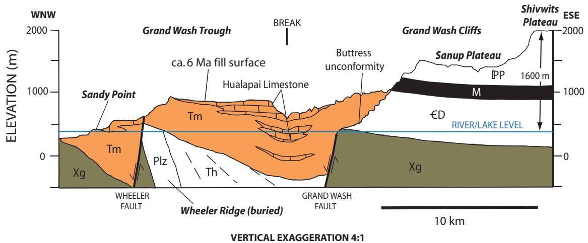
Figure 3. Cross section showing stratigraphic and structural relations at the western terminus of Grand Canyon. Section to the left of the break is modified after Wallace et al. (2005), and section to the right of the break is modified after Billingsley et al. (2004). Xg—Proterozoic basement; €D—Cambrian through Devonian strata; M—Mississippian strata; PP—Pennsylvanian and Permian strata; Plz—Paleozoic strata undifferentiated; Th—Horse Spring Formation; Tm—Muddy Creek Formation (sedimentary rocks of Grand Wash Trough). See Figure 2 for location of section.
