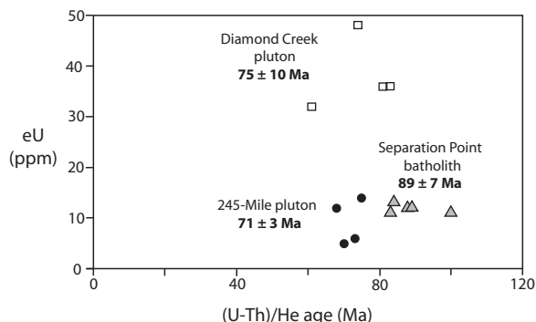
Figure 5. Plot of single-grain apatite (U-Th)/He ages versus effective uranium concentration for three Lower Granite Gorge basement samples (data from Flowers et al., 2008). Sample locations are on Figure 2, keyed by age.
