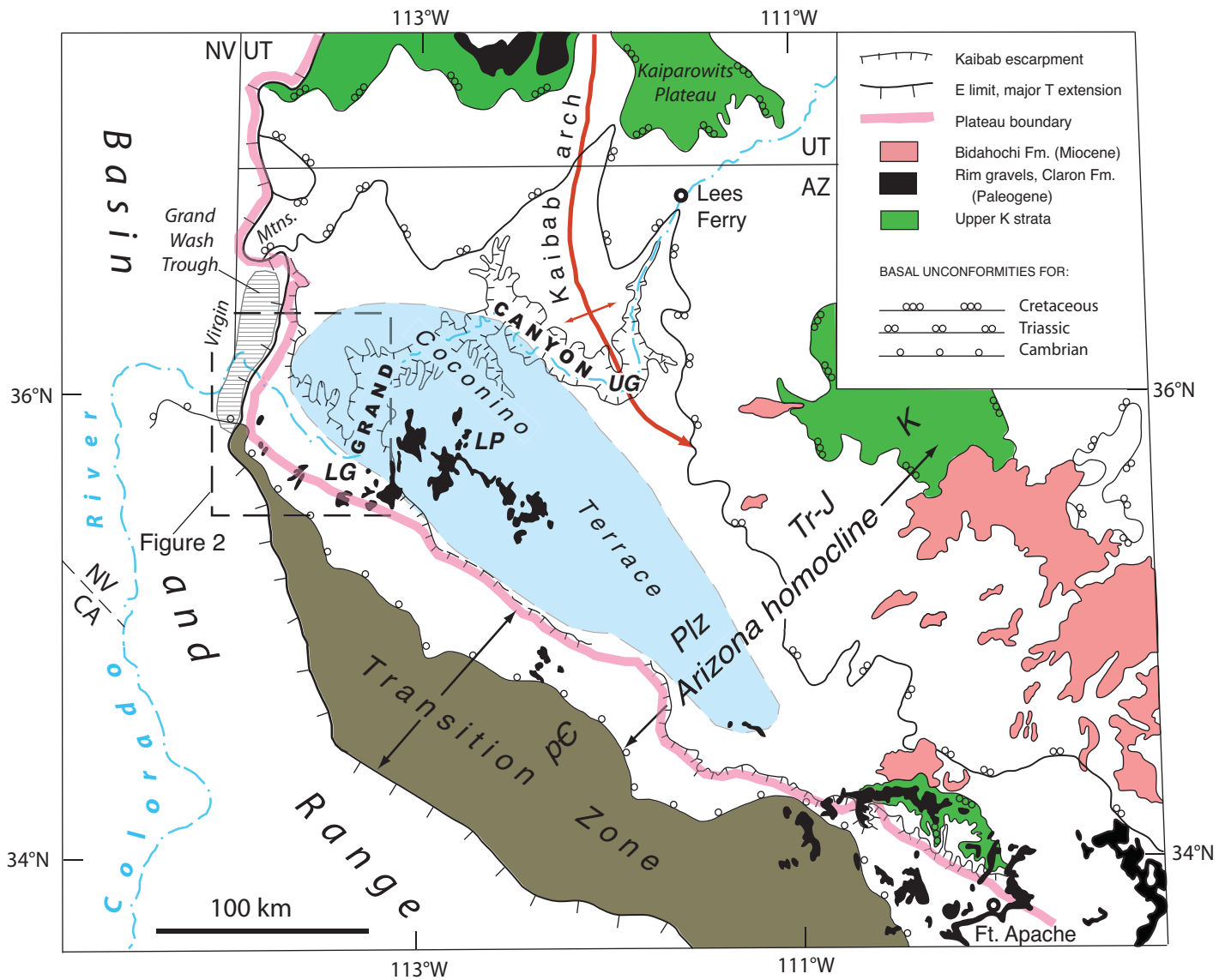
Figure 1. Tectonic map showing selected geographical and geological features discussed in text. Geology of Colorado Plateau and Transition Zone is generalized with late Cenozoic volcanic units removed. Boundary of Coconino terrace (light-blue area), based on regional elevation of the top of the Kaibab Formation at 1600 \pm 200 m, is based on contour map of Hunt (1969). LG—Lower Granite Gorge of Grand Canyon; LP—Long Point area; UG—Upper Granite Gorge; pC—Proterozoic crystalline and overlying Proterozoic stratified rocks; Plz—Paleozoic strata; Tr-J—Triassic and Jurassic strata; K—Cretaceous strata.
