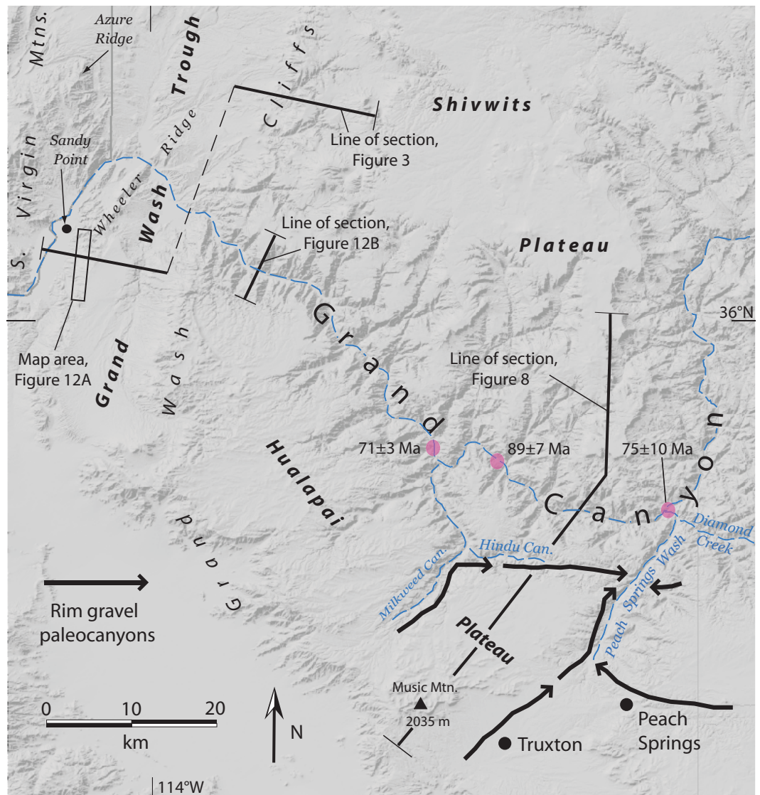
Figure 2. Shaded relief map of western Grand Canyon–Lower Granite Gorge region showing locations of sections and map in Figures 3, 8, and 12, the location of paleocanyons (generalized from Young, 2008), sample locations of the three (U-Th)/He apatite ages shown in Figure 5 and discussed in text (magenta circles; after Flowers et al., 2008), and selected geographical features discussed in text.
