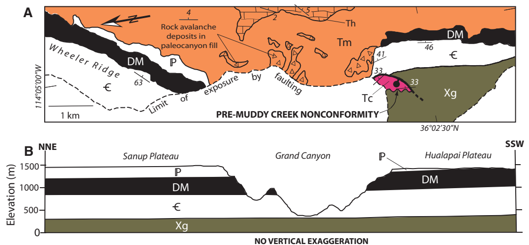
Figure 12. (A) Geologic map of Wheeler Ridge paleocanyon, simplified from Wallace et al. (2005); lines with tick marks and numbers show strike and dip of bedding. (B) Cross section through western Grand Canyon for comparison, using geology from Wenrich et al. (1996). See Figure 2 for location of map and section. Xg—Proterozoic crystalline basement; €—Cambrian strata; DM—Devonian–Mississippian strata; P—Pennsylvanian strata; Tc—Tertiary conglomerate and intercalated ash beds with sandine yielding an Ar–Ar age of 15.3 \pm 0.1 Ma; Tm—Muddy Creek Formation (sedimentary rocks of Grand Wash Trough); Th—Hualapai Limestone.
