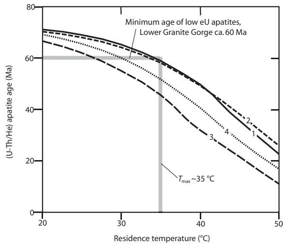
Figure 6. Curves showing apatite (U-Th)/He model age as a function of temperature for samples cooled rapidly from 120 °C and held isothermally for 70 m.y., for apatites with properties similar to the 245-Mile pluton sample (Figs. 2 and 5; eU = 14 ppm; grain radius = 60 \mu m), using the radiation damage and annealing model (RDAAM) of Flowers et al. (2009). Curves labeled 1–4 correspond to parameter sets 1–4 given in table 1 of Flowers et al. (2009). All parameter sets predict ages younger than 60 Ma for residence temperatures above 35 °C.
