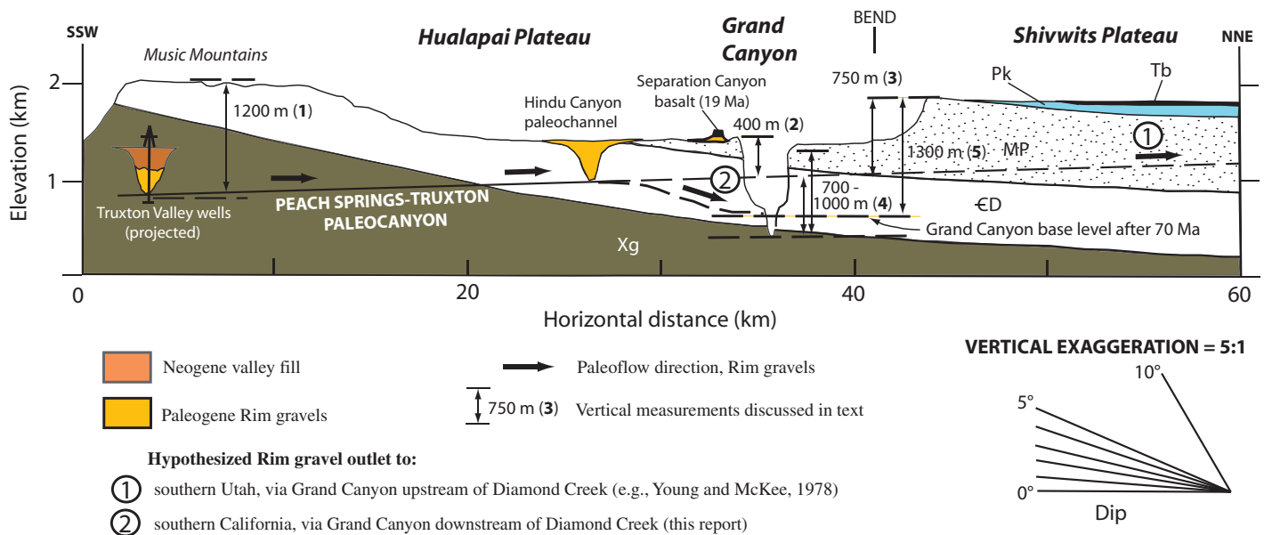
Figure 8. Cross section through the western Grand Canyon region showing geometric relationships between various geomorphic and geologic features discussed in text (based on Young, 1982). Xg—Proterozoic crystalline basement; CD—Cambrian and Devonian strata; MP—Mississippian to Permian strata; Pk—Permian Kaibab Formation; Tb—8 Ma Shivwits basalts. Vertical arrows show measurements of elevation differences discussed in text. Hindu Canyon channel depicted assuming present minimum elevation of Rim gravel deposits in Peach Springs Wash (1000 m) has not been modified by faulting (see text for discussion).
