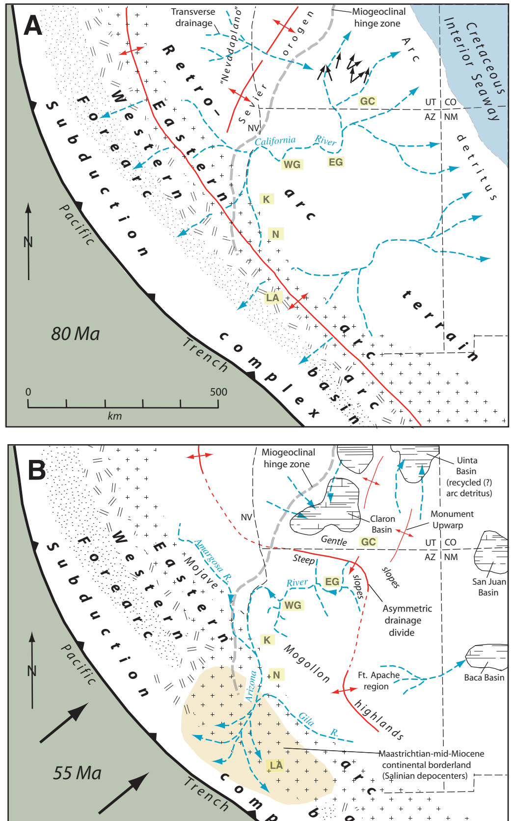
Figure 9. Paleogeographic maps showing: (A) Campanian position of California River drainage near the onset of incision in the Grand Canyon region. Red line shows position of drainage divide; black arrows show paleocurrent directions of the Wahweap Sandstone from Lawton et al. (2003), along with hypothetical position of drainage transverse to the Sevier orogen. Sevier uplands and hypothetical “Nevadaplano” high plateau are from DeCelles (2004). (B) Early Eocene positions of Arizona River drainage, the drainage system in the Fort Apache region (Potochnik, 2001), and ancestral Gila and Amargosa Rivers (Howard, 1996). Palinspastic base and direction of plate convergence are after Saleeby (2003). Position of drainage divide in Nevada is from Henry (2008). Abbreviations highlighted with yellow background correspond to locations in Figure 13 as follows: LA—Los Angeles; N—Needles; K—Kingman–Lake Mead area; WG—western Grand Canyon; EG—eastern Grand Canyon; GC—Glen Canyon.
