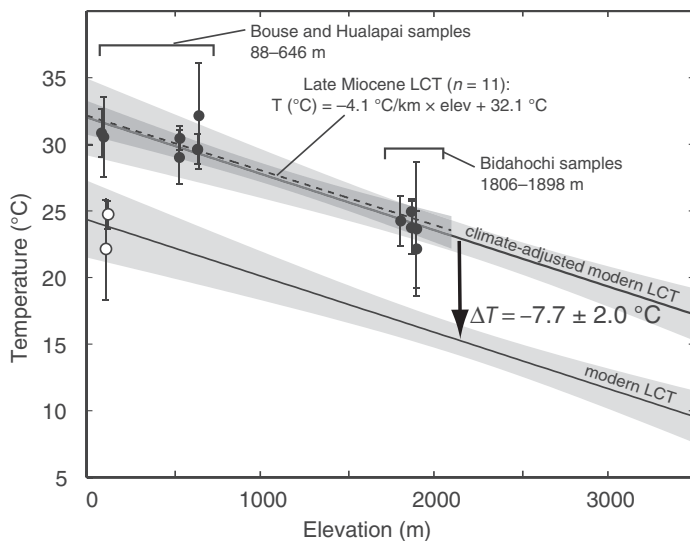
Figure 7. Carbonate clumped-isotope thermometry temperature estimates versus modern elevation for samples collected in the Colorado River basin (after Huntington et al., 2010). Data points marked by unfilled circles are interpreted to reflect cooling of lake surface temperatures due to the influence of marine climate near the late Miocene delta. Inland samples define a lacustrine carbonate temperature (LCT) lapse rate for the late Miocene similar to the modern LCT lapse rate, suggesting little or no elevation adjustment of the southwestern Colorado Plateau since 16 Ma. Vertical arrow shows apparent 8 °C of cooling of lake depositional temperatures since 6 Ma, interpreted to reflect climatic cooling.
