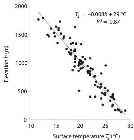
Figure 11. Plot of surface temperature versus elevation in shallow boreholes throughout the southwestern United States. Plot was constructed by extrapolating temperature-depth curves (figs. A2 through A8 in Sass et al., 1994) to Earth's surface. Regression equation assumes h in meters.
