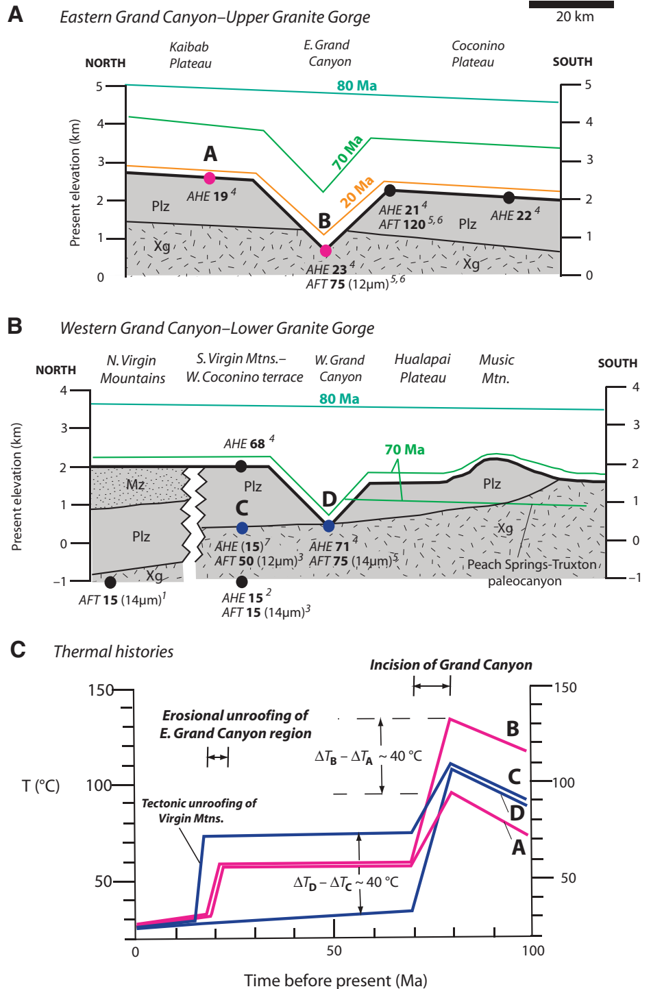
Figure 4. Schematic cross sections showing representative thermochronological data, low-temperature thermal histories, and erosion histories for Grand Canyon region. Erosion histories assume a geothermal gradient of 25 °C/km. (A) Section showing positions of rim and gorge samples (circles) and inferred position of the erosion surface (colored lines) at the times indicated on the curves in the eastern Grand Canyon region. AHE—(U-Th)/He apatite age; AFT—fission-track apatite age, showing mean track lengths in parentheses. Here, representative ages shown are not averages of measured ages, but calculated times of rapid cooling through most or all of the AFT partial annealing zone or AHE partial retention zone, as discussed in text. (B) As in A for western Grand Canyon; ages for point D are from the Diamond Creek area, where both AHE and AFT data exist. Sources of data: 1—Quigley et al. (2010); 2—Reiners et al. (2000); 3—Fitzgerald et al. (1991, 2009); 4—Flowers et al. (2008); 5—Kelley et al. (2001); 6—Dumitru et al. (1994); 7—age inferred from structural position between the surface and the base of the partial annealing zone for apatite fission tracks (Fitzgerald et al., 1991; Reiners et al., 2000). (C) Cooling histories for the four lettered sample positions in A and B, and discussed in text.
