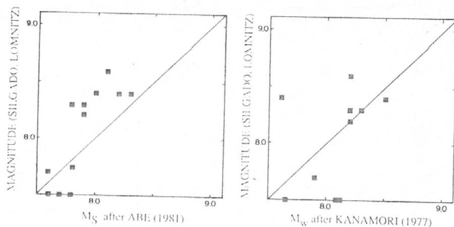
FIG. 3. A comparison between Lomnitz or Silgado magnitudes and either M_S (Abe, 1981; Abe and Noguchi, 1983) or M_W (Kanamori, 1977).
