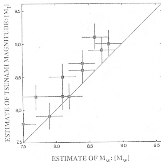
FIG. 7. A comparison between the estimates [M_w] for M_w and [M_t] for M_t for Peruvian historical earthquakes. The values of [M_t] are somewhat higher than [M_w] , but the difference of 0.2 is not statistically significant. The slope is unity.
