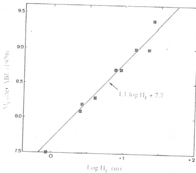
FIG. 5. Linear regression between the tsunami magnitude M_t (after Abe, 1979) and the local wave height H_r(m) for South American earthquakes. The small dispersion for South America contrasts with the large scattering shown by Abe when all regions are included.
