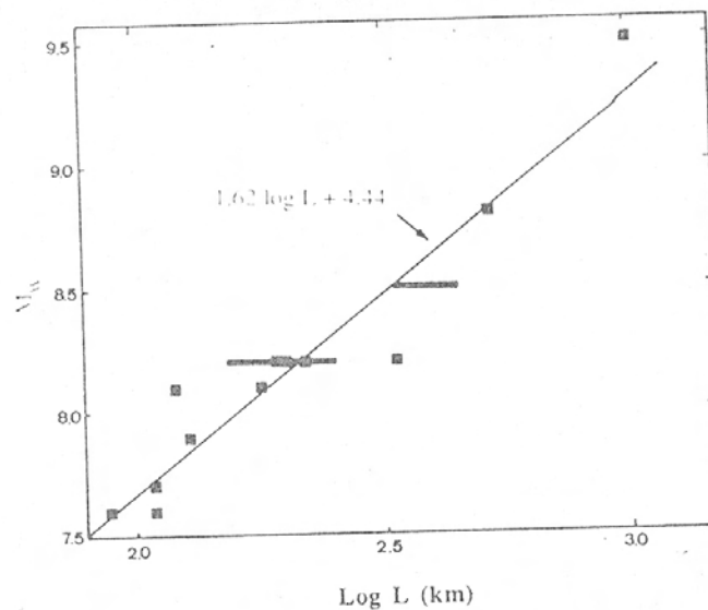
FIG. 4. M_w against \log L (rupture length in km) for several South American earthquakes of this century. Data from Kanamori (1971), Kanamori and McNally (1982), Kelleher (1972), and Nishenko (1985).
