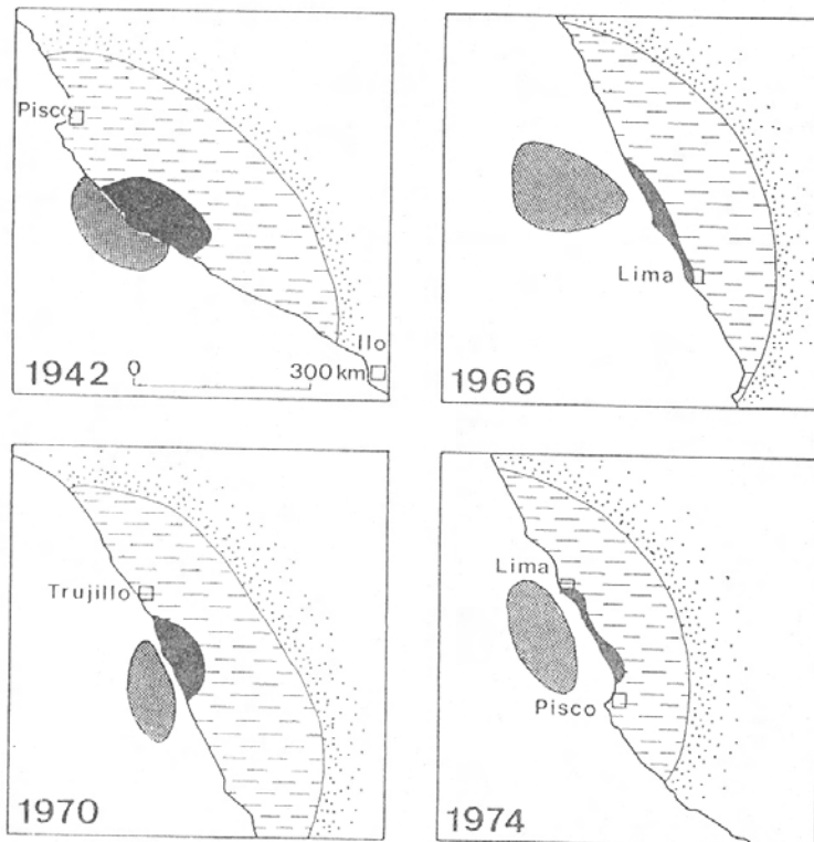
FIG. 2. Test earthquakes (1942, 1966, 1970, and 1974) for a comparison between the aftershock area (gray) and the isoseismal of intensity VIII (black) or zone 1. Horizontally hatched region is zone 2, and dotted region is zone 3.
