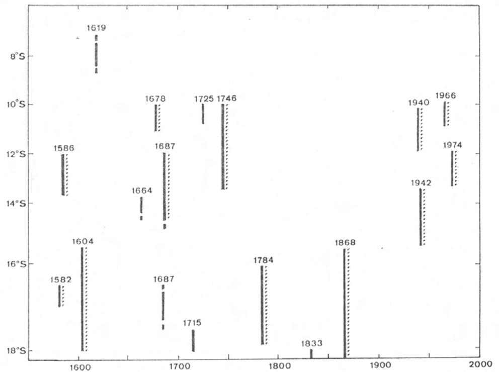
FIG. 6. Rupture zones of historical earthquakes in Peru as a function of time. The scale of latitude varies because length is measured along the trench and not along a meridian. The wavy symbols indicate tsunamogenic earthquakes. Three zones are clearly delimited in latitude.
